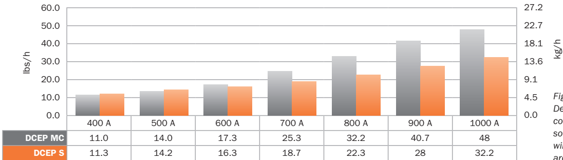
4.0 mm (5/32") Diameter wire Comparisons (DCEP)
