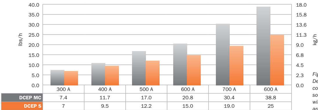
4.0 mm (5/32") Diameter wire Comparisons (DCEP)
